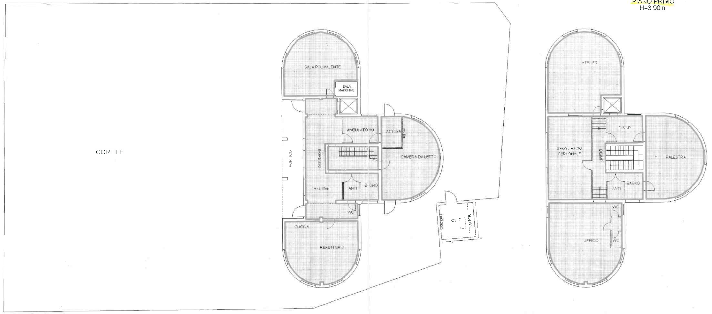
PIANO TERRA H=3.85m
